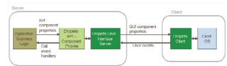
Figure 2: Overview of the Droplets RIA architecture
